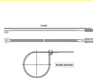
CST100 37/48-B 370X4.8mm
