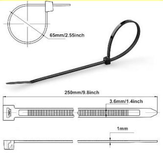
CST100 25/36-N 250X3.6mm
