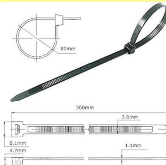
CST100 30/36-N 300X3.6mm
