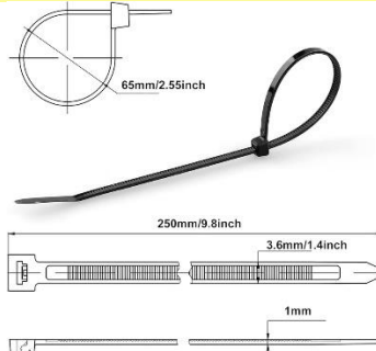
CST100 20/36-N 200X3.6mm
