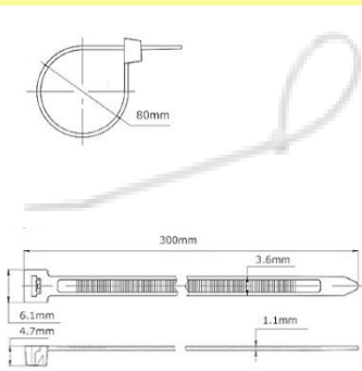
CST100 30/36-B 300X3.6mm
