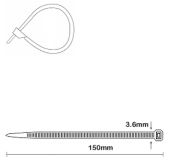
CST100 15/36-N 150X3.6mm
