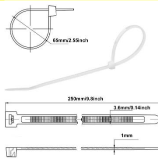
CST100 25/36-B 250X3.6mm
