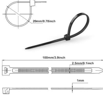
CST100 10/25-N 100X2.5mm
