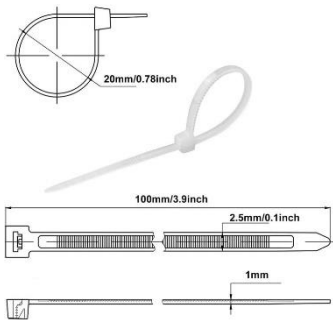
CST100 10/25-B 100X2.5mm
