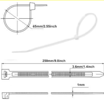
CST100 20/36-B 200X3.6mm
